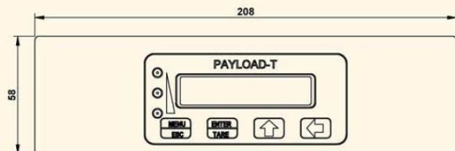
ELEVATION GA OF PAYLOAD TIPPER
